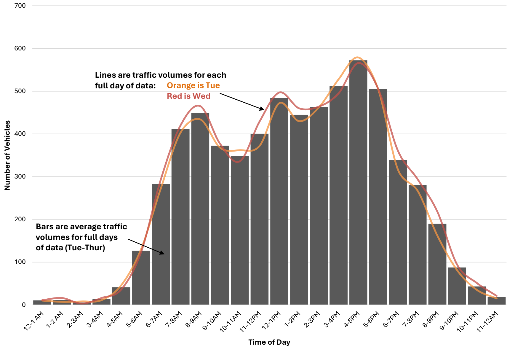
Daily Traffic Profile at NH 103/NH 127 (Park Ave) over Contoocook River (both ways)
